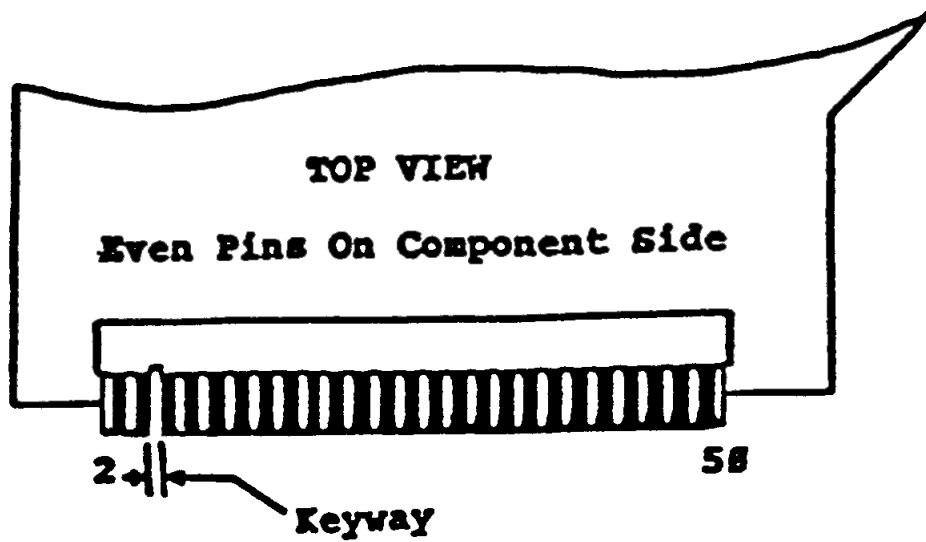
INTERFACE CONNECTOR
